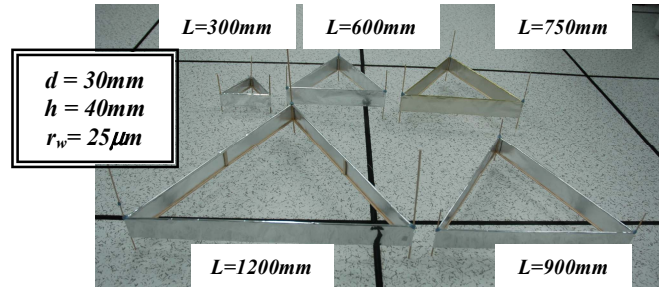
Figure 8. Five Ionic Flyers with L = 300mm , 600mm , 750mm , 900mm and 1200mm
