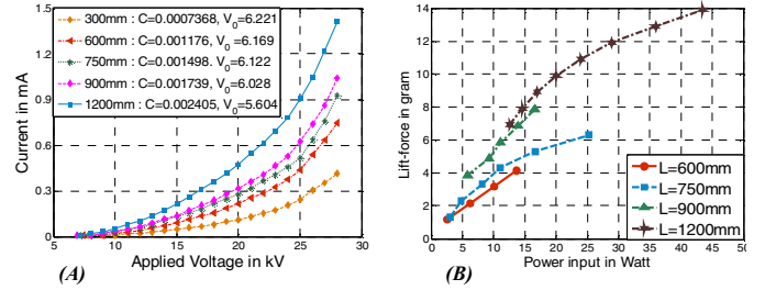
Figure 9. (A) I - V curves and (B) F - P curves for the Ionic Flyers with L = 300mm , 600mm , 750mm , 900mm and 1200mm
